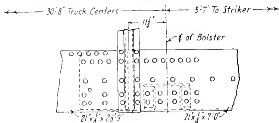
Fig. 4—Detail of Splice for Sides of Steel Coal Cars
